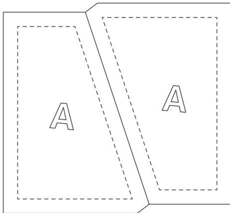
A Shapes (layer fabrics and cut at the same time)
